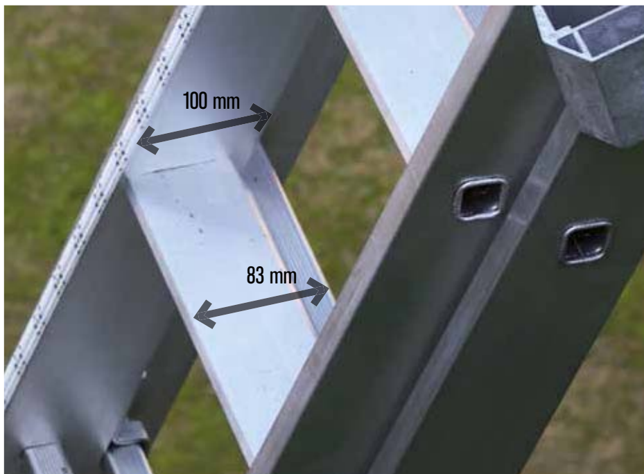
Gradino anteriore largo 83 mm. 83 mm wide front step.
